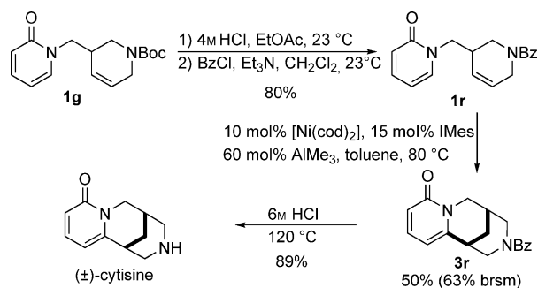
Scheme 2. Application of the endo -cyclization mode for the synthesis of the lupin alkaloid (±)-cytosine. brsm = based on recovered starting material, Bz = benzoyl.
