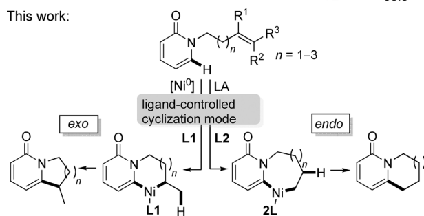
Scheme 1. Intramolecular 2-pyridone hydroarylation. cod = 1,5-cyclo-octadiene.
