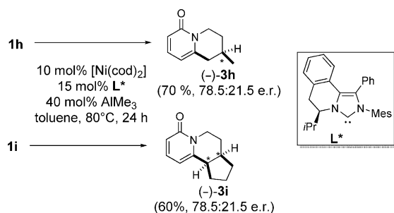
Scheme 3. Preliminary results towards a catalytic asymmetric version of the endo cyclization with a chiral NHC ligand.
